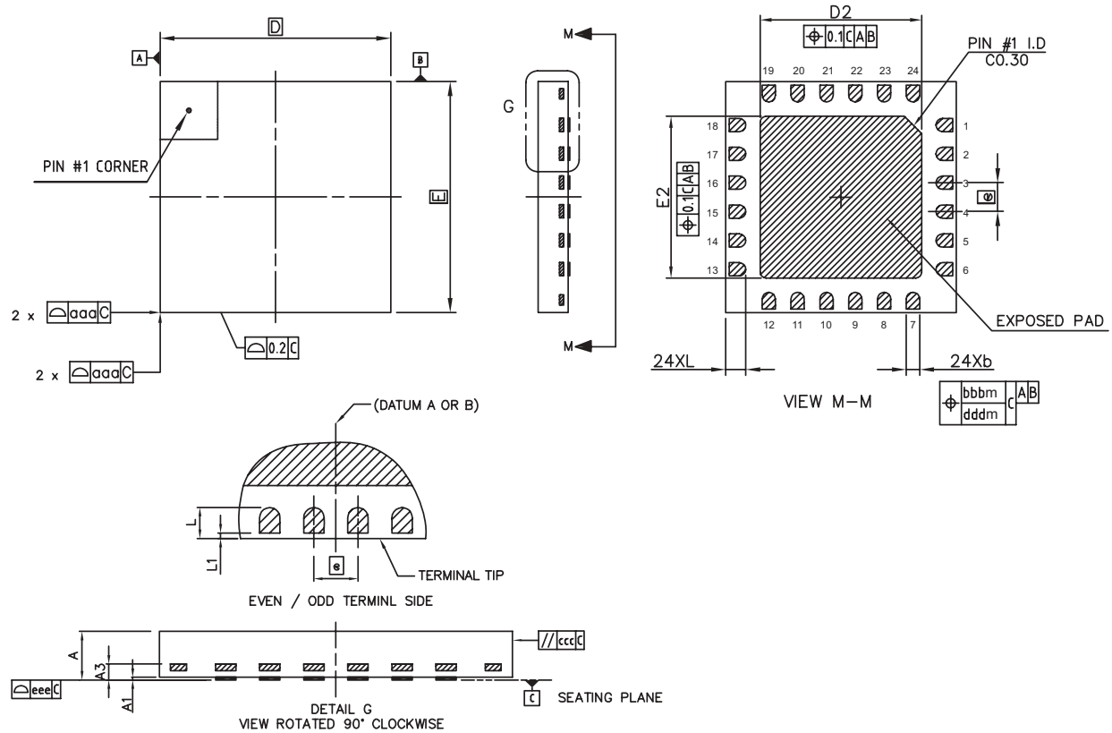
Figure 20. TQFN(4x4)-24 Package
