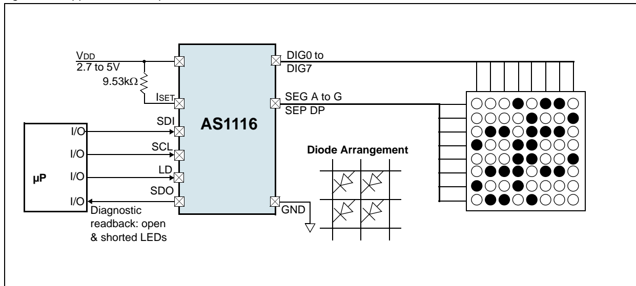
Figure 18. Application Example as LED Dot Matrix Driver
