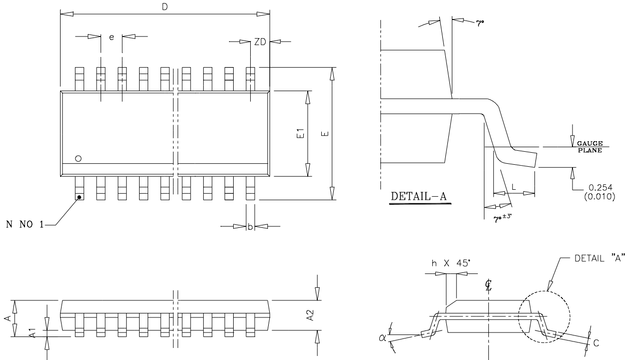
Figure 19. QSOP-24 Package
