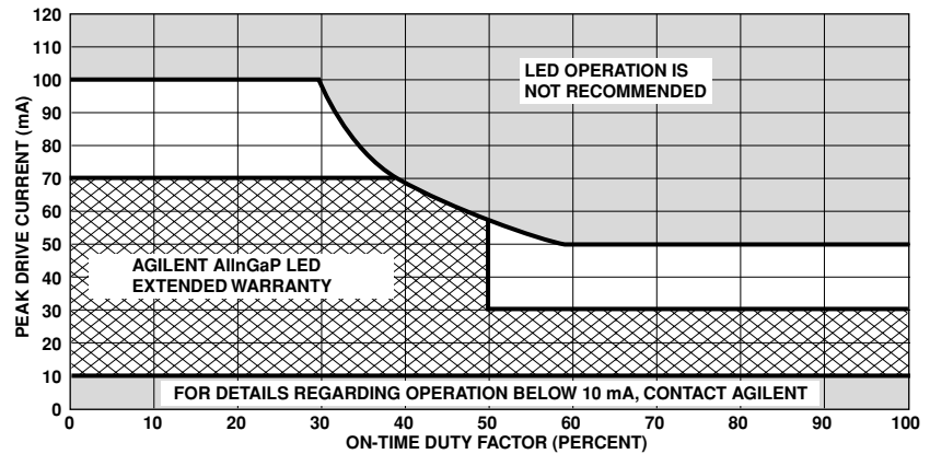
Figure 6. Avago Technologies AlInGaP LED Extended Warranty Pulsed Current Operating Range
