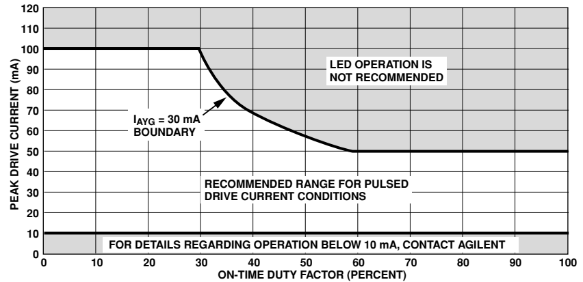
Figure 2. Recommended Range for Pulsed Drive Current Conditions for AllInGaP LEDs
