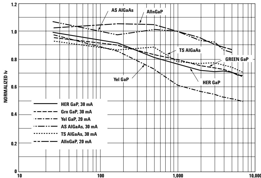
Figure 8. Typical Reduction in Luminous Intensity for Agilent Technologies GaP, AlGaAs, and AlInGaP LEDs.
