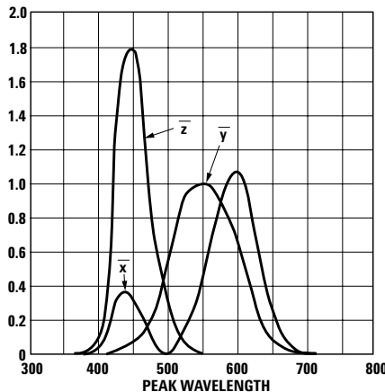
Figure 17. 1931 CIE Color Matching Functions.
