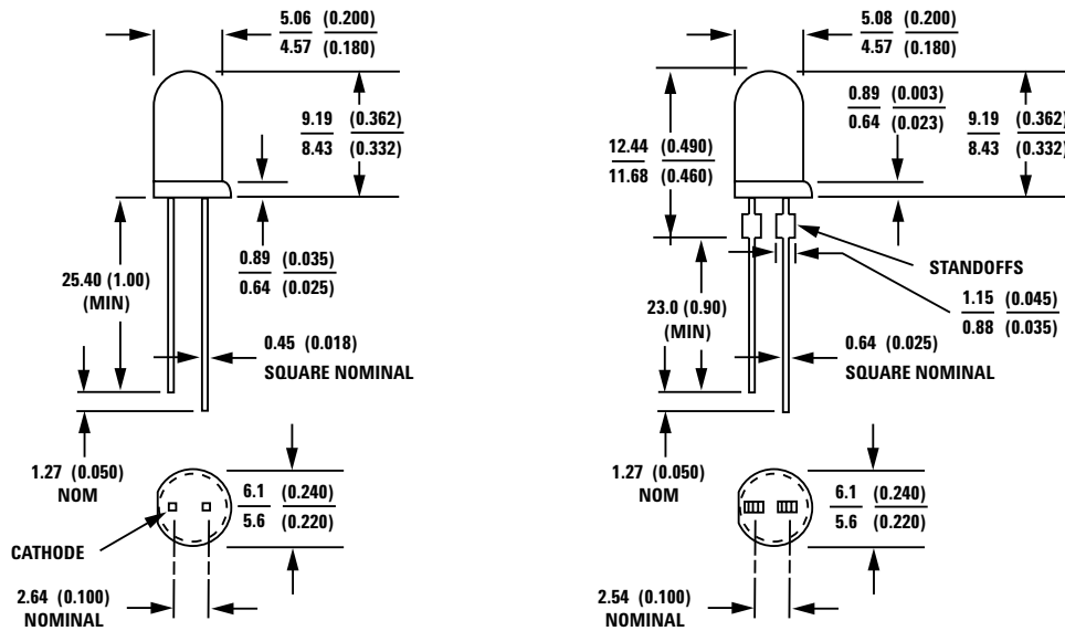
Figure 5. T-1 3/4 LED Lamp Package Outlines.
