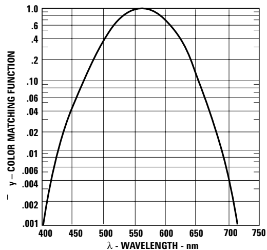
Figure 12. 1931 CIE y Color Matching Function.
