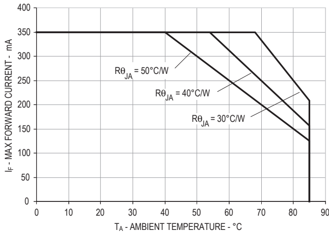
Figure 11. Maximum forward current vs. ambient temperature for InGaN Deredated based on T_{jMAX} = 110^{\circ}C , R_{\theta_{JA}} = 30^{\circ}C/W / 40^{\circ}C/W and 50^{\circ}C/W
