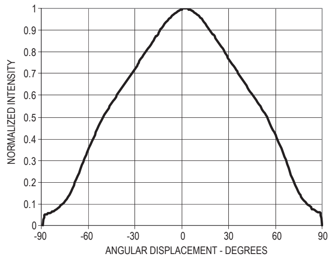
Figure 10. Radiation Pattern – Major Axis
