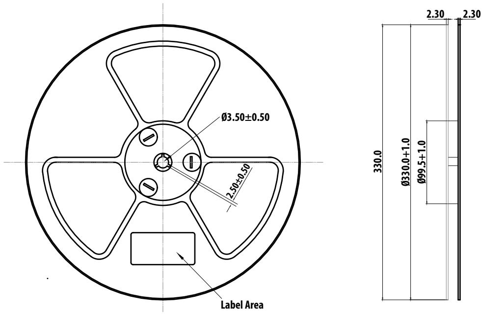
Figure 15. Reel Dimension
