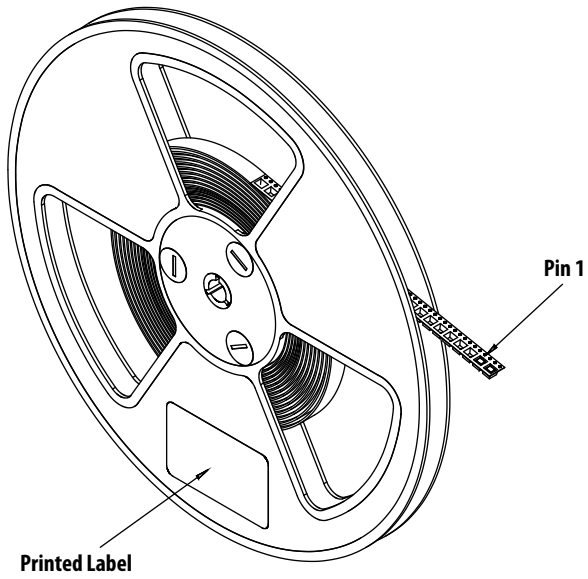
Figure 16. Reeling Orientation
