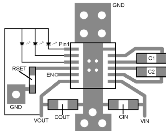
Figure 3. Recommended Layout
