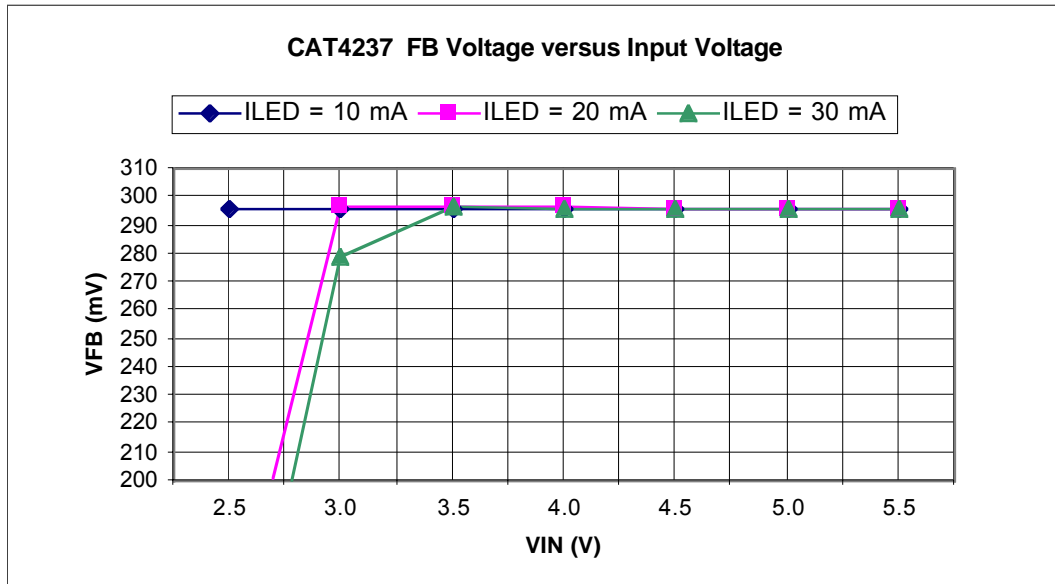
Figure 6. V FB Voltage Line Regulation
