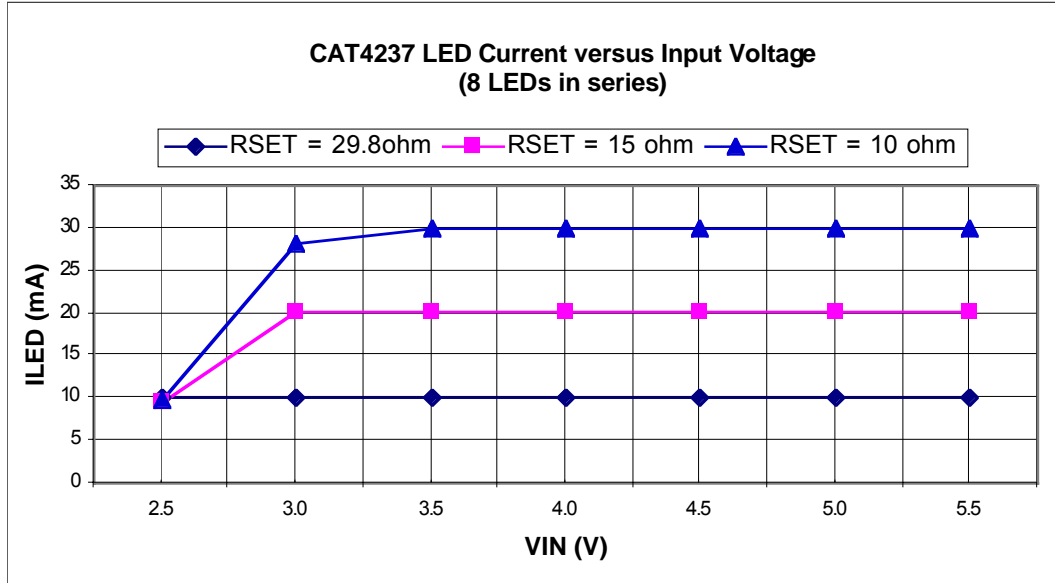
Figure 5. LED Current Line Regulation
