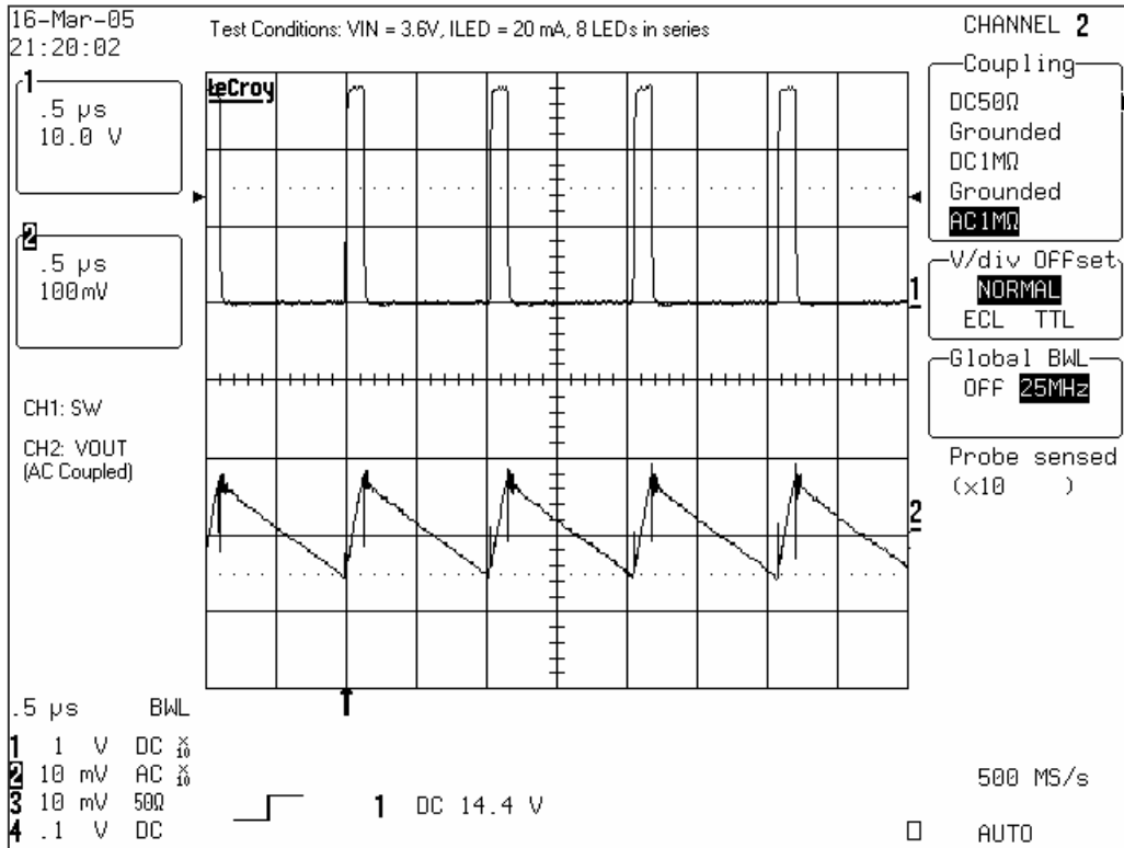
Figure 4. Internal Switch and Output Voltage Waveforms ( V_{IN} = 3.6\text{V} , I_{LED} = 20\text{mA} )
