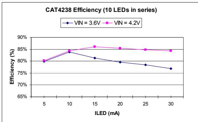
Figure 6. CAT4238 Efficiency driving 10 LEDs in series
