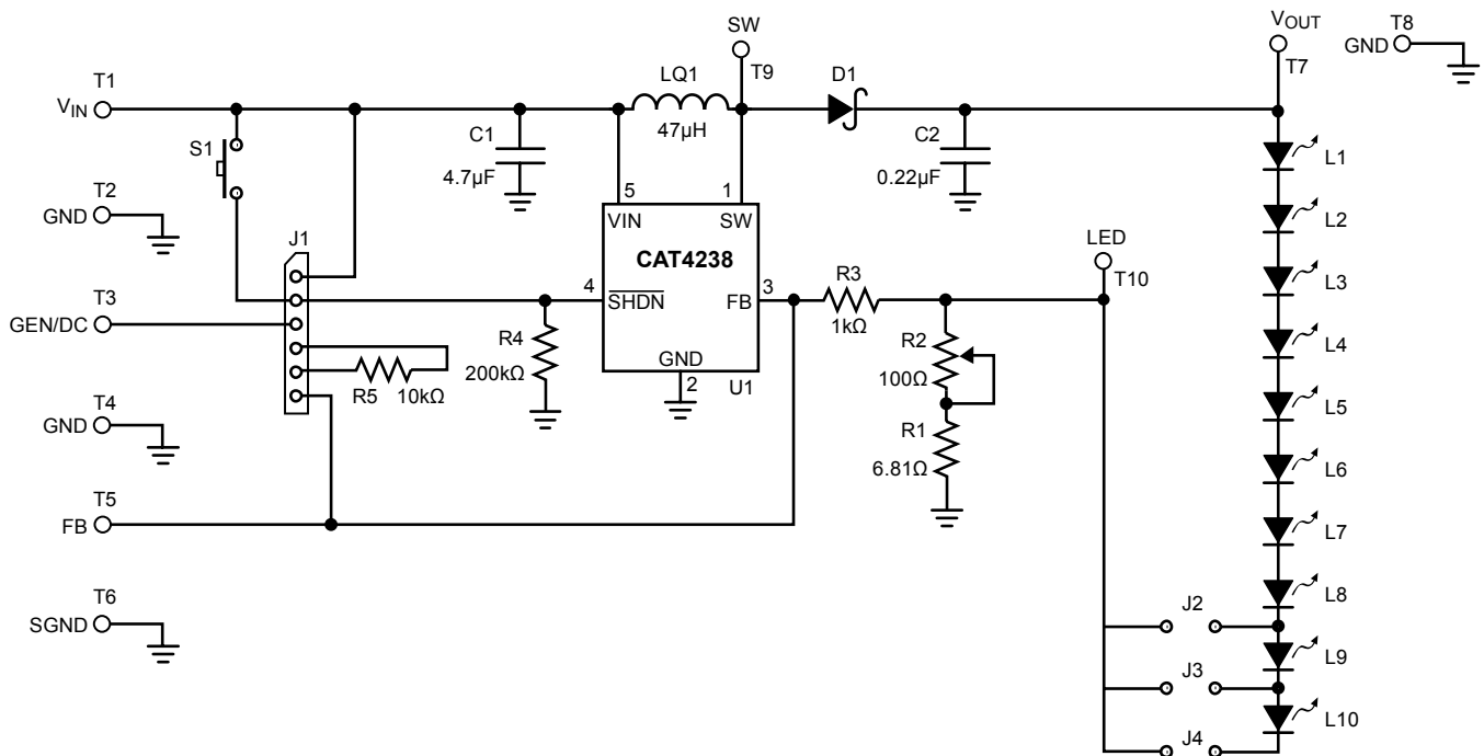
Figure 1. CAT4238EVAL1 Board Schematic
