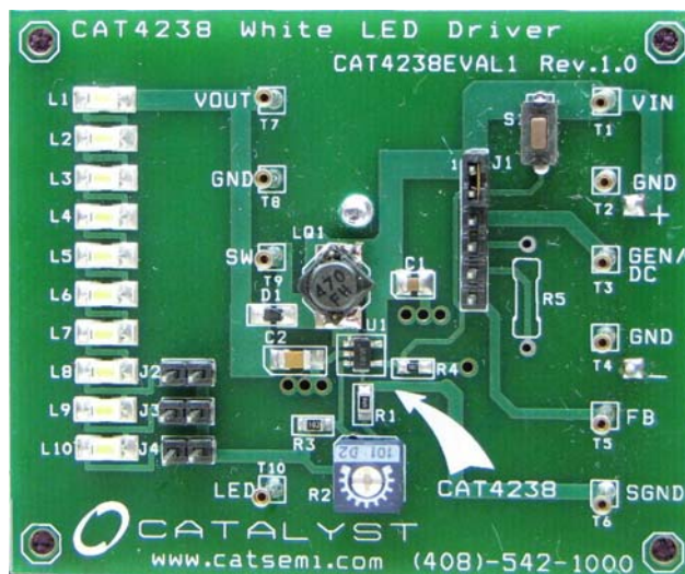
Figure 2. CAT4238EVAL1 Board
