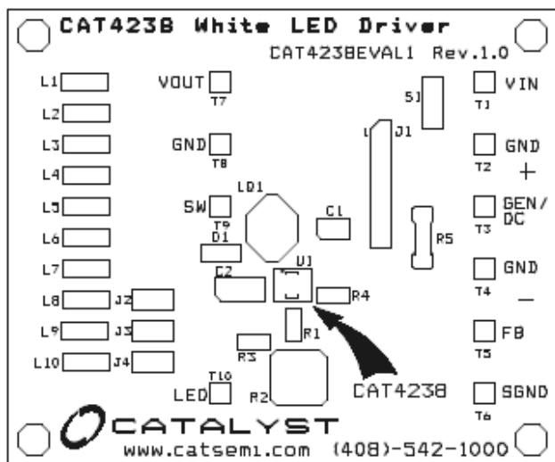
Figure 2. CAT4238EVAL1 Board
