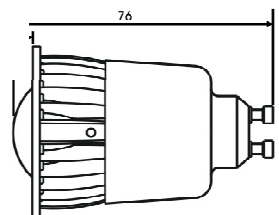
TRISTAR-GU10-L with lens. It has a beam angle of 30°.
