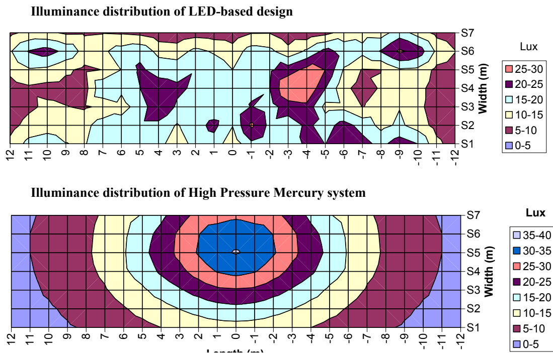
Figure 4: Light Distribution of LEDs versus Mercury Vapor
