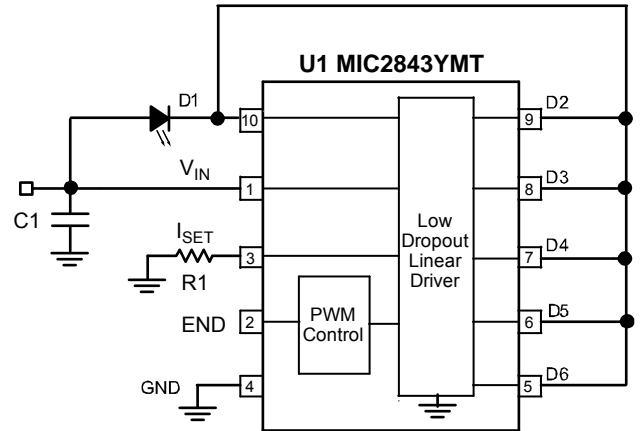
Figure 11. Six Channel (Parallel) Application Circuit
