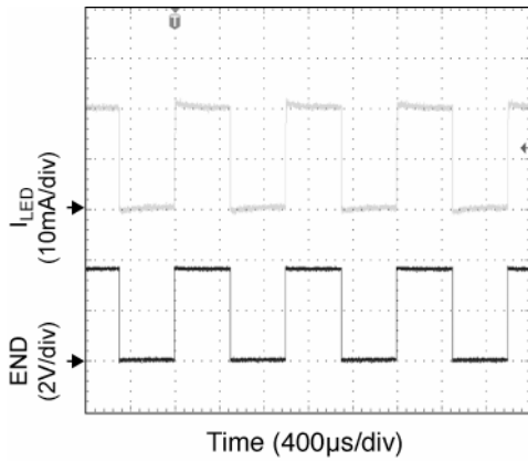
Figure 8. PWM Signal at 50% Duty Cycle ( I_{avg} = 10mA )
