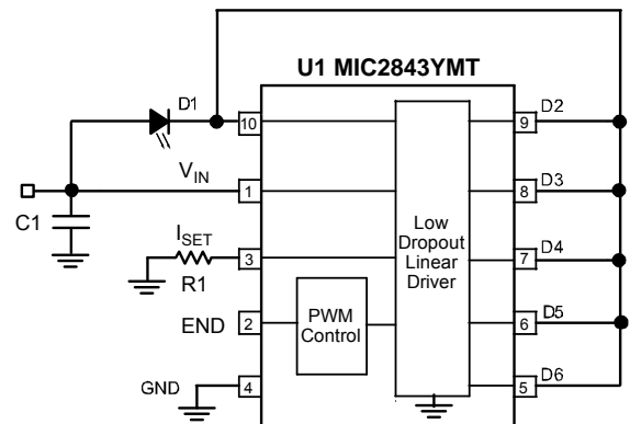
High Current Flash Driver
