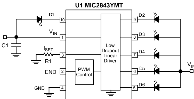
LCD Display Backlight with Six WLEDs
