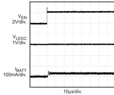
Startup in 1x Mode 3 x 10mA LEDs
