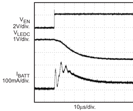
Startup in 1.5x Mode 3 x 10mA LEDs
