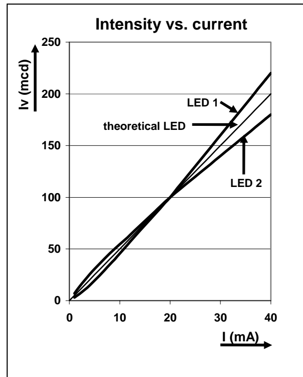
Figure 1 - LED I/v curve
