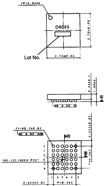
VCSP50L3 (35pin) (Unit : mm)
