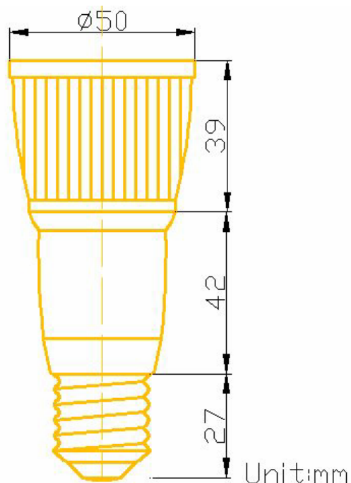
RP-SL-H02-10WXXE27
