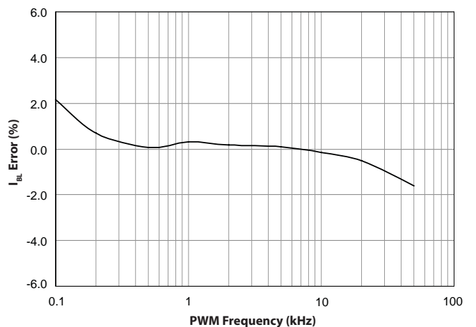
I_{BL} Error vs. PWM Frequency at 50% Duty Cycle
