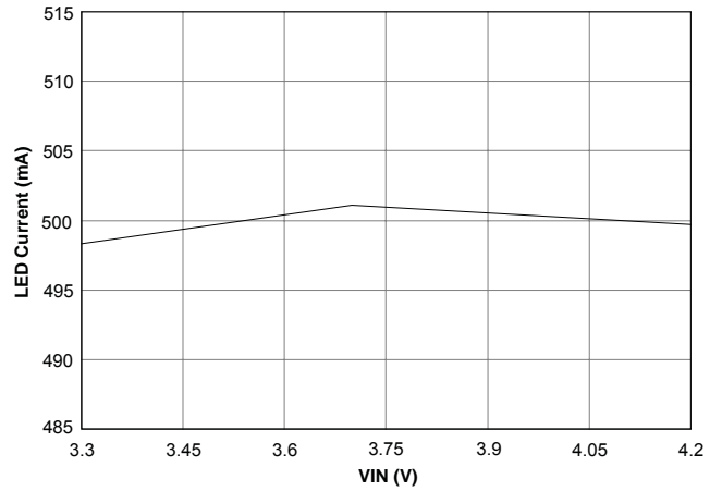
Spotlight Current, R_{ISET} = 500m\Omega , V_{OUT} = 2.93V
