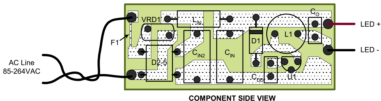
Figure 7. Recommended circuit board layout with the HV9923N3
