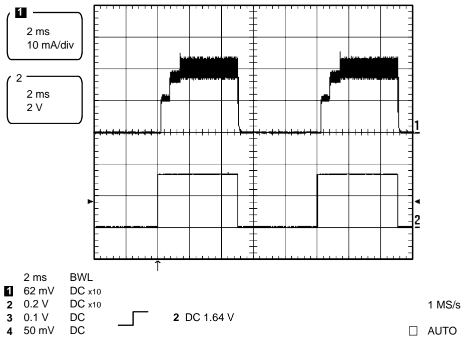
Figure 2–8. Output Current vs Duty Cycle for PWM Dimming Using Enable
