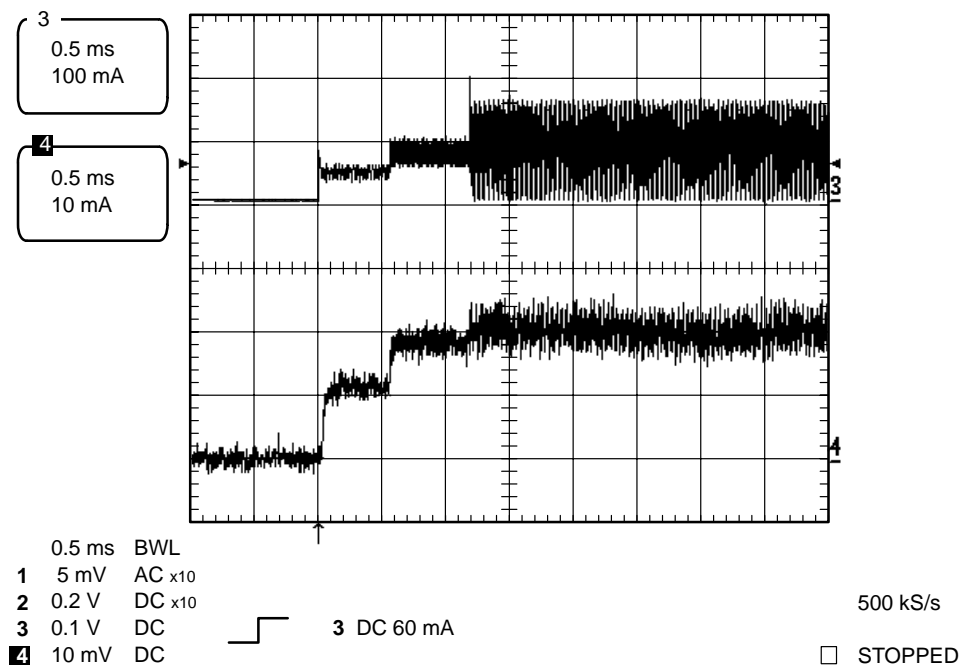
Figure 2–1. Startup Waveforms
