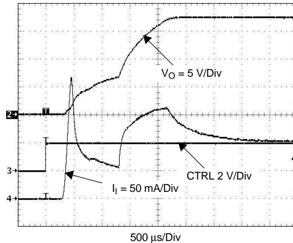
Figure 15. . Soft Start
