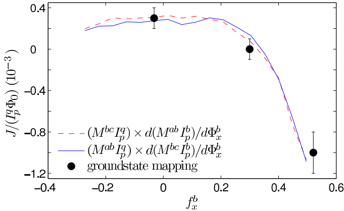
FIG. 5: Coupling strength (in units of coupled flux) versus f_x^b as obtained from groundstate mapping and from dM^{ab} I_p^q / d\Phi_x^b scaled by M^{ab} I_p^q with I_p^q = (0.5 \pm 0.1) \mu\text{A} [see Eq. (1)].
