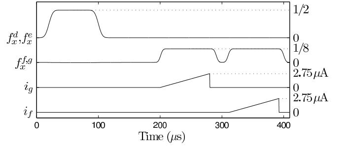
FIG. 2: Bias sequence. CJJ biases f_x^d, f_x^e are raised to \frac{1}{2} , held for 60 \mu\text{s} , and then returned to zero over 20 \mu\text{s} . Readout dc-SQUID flux bias f_x^{f,g} is held at zero during qubit evolution and raised to its operating point during the current bias ramps on i_f, i_g . Control lines f_x^a, f_x^b , and f_x^c are held constant throughout this procedure.
