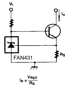
Figure 17. Constant-Current Sink
