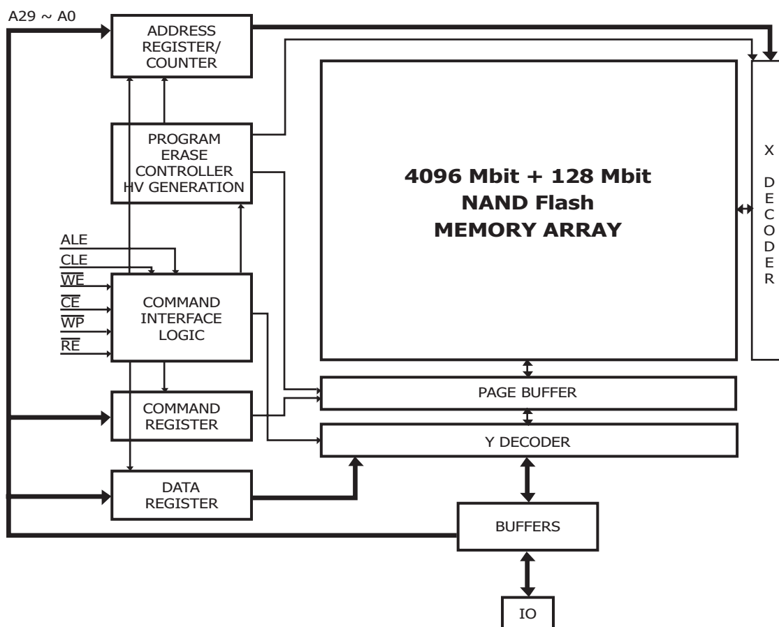
Figure 3: Block Diagram
